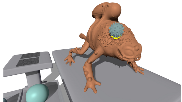
Figure 9: Deformation on a subdivision surface with existing displacements using a pen-device-controlled sculpting geometry. For constraining the penetration depth, the pressure of the pen device is used to apply forces to the tool controlled by the physics engine.
