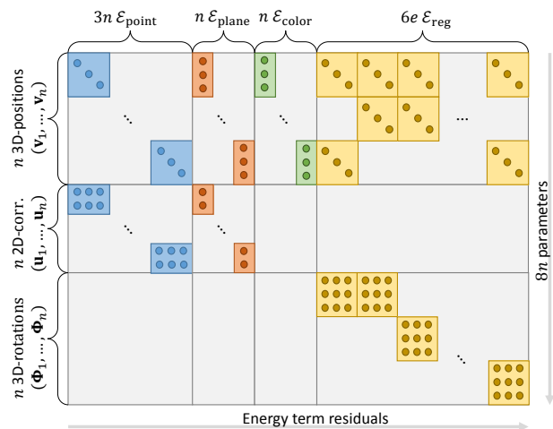
Figure 5: Block structure of the (\mathbf{V}, \mathbf{U}, \Phi) Jacobian (transposed). The Jacobian is never stored explicitly; instead the products J\mathbf{h} and J^\top\mathbf{h} are computed on demand on the GPU.
