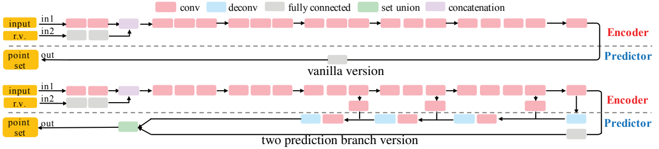
Figure 2. PointOutNet structure
