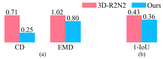
Figure 6. Quantitative comparison to 3D-R2N2. (a) Point-set based metrics CD and EMD. (b) Volumetric representation based metric 1-IoU. Lower bars indicate smaller errors. Our method gives better results on all three metrics.
