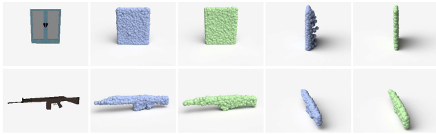
Figure 13. Comparison of predictions of networks trained by CD (blue, on the left) and EMD (green, on the right).
