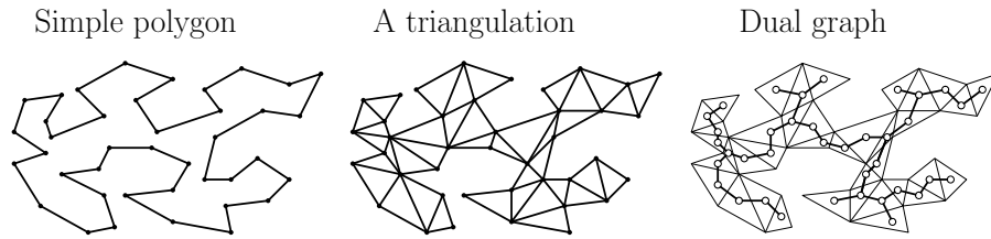
Fig. 24: Polygon triangulation.
