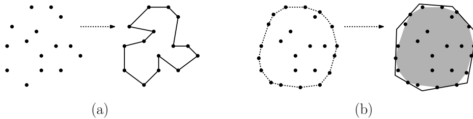
Fig. 79: Geometric approximations: (a) Euclidean traveling salesman, (b) approximate convex hull.
