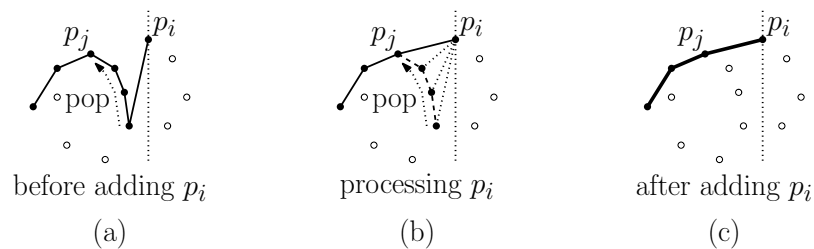
Fig. 13: Graham's scan.
