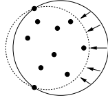
Fig. 104: Contact points for a minimum enclosing disk.
