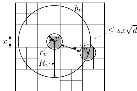
Fig. 86: WSPD analysis.
