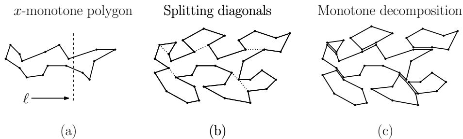
Fig. 25: Monotonicity.
