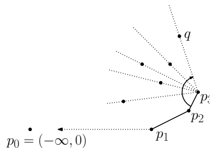
Fig. 15: Jarvis's march.
