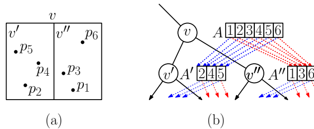
Fig. 78: Cascaded search in range trees.
