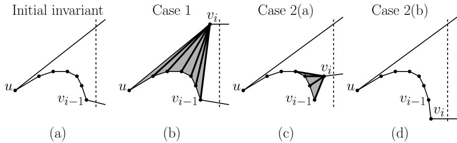
Fig. 27: Triangulation cases.
