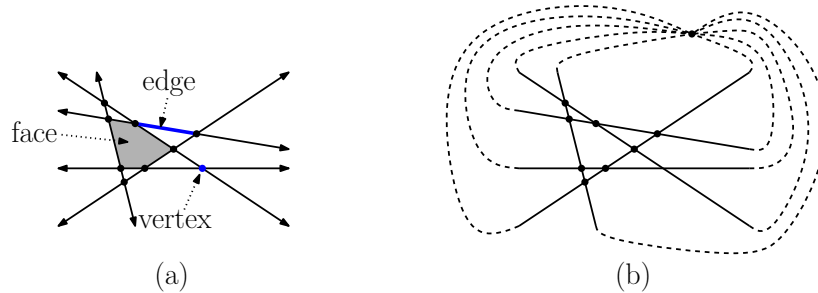
Fig. 62: Arrangement of lines; (a) the basic elements of an arrangement and (b) adding a vertex at infinity to form a proper planar graph.
