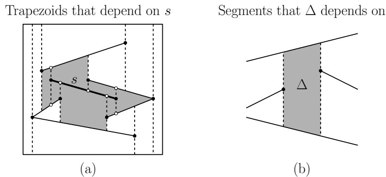
Fig. 42: Trapezoid-segment dependencies.
