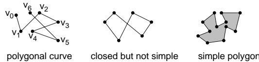
Fig. 154: Polygonal curves
