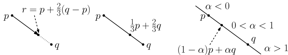
Fig. 99: Affine combination.
