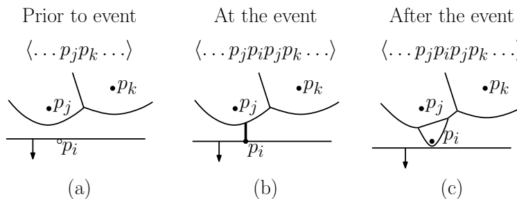
Fig. 51: Site event.
