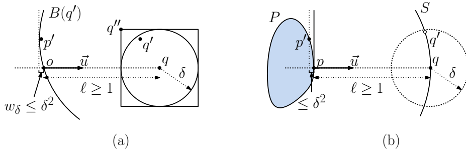
Fig. 97: Analysis of the coresets construction.
