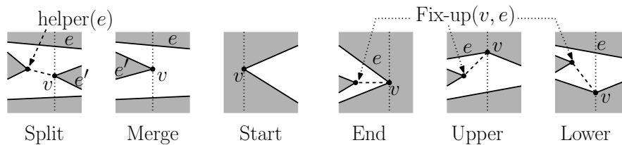
Fig. 29: Plane sweep cases, where v is the vertex being swept. The label e denotes the edge such that helper(e) \leftarrow v .
