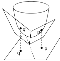
Fig. 123: Intersection of halfspaces.
