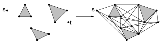
Fig. 129: Visibility graph.
