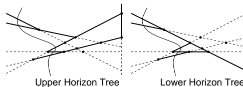
Fig. 126: Upper and lower horizon trees.
