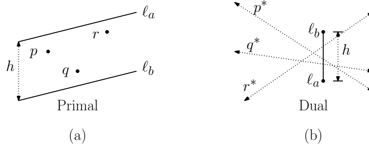
Fig. 67: A 3-corridor in the (a) primal and (b) dual form. (Note that the corridor is not as narrow as possible.)
