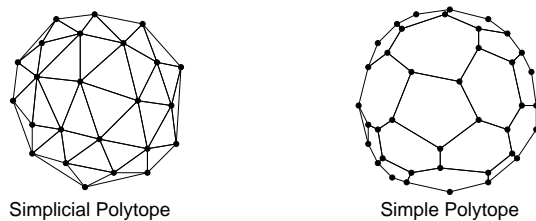
Fig. 150: Simplicial and simple polytopes.
