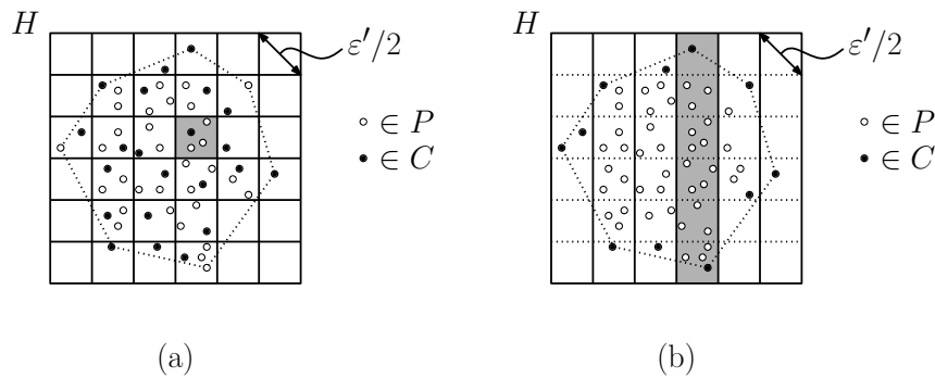
Fig. 95: The quick-and-dirty coresets construction: (a) of size O(1/\varepsilon^d) and (b) the improved construction of size O(1/\varepsilon^{d-1}) .
