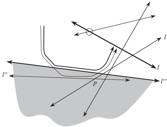
Figure 14: The fact that line l'' charges line l' in one bay traversal implies that l'' shields the portion of l' (darkened) to the left of point p from being touched by any previous bay traversal.
