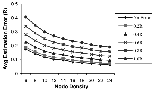
Figure 23: Target estimation error with different localization errors under varying node density
