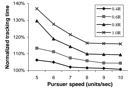
Figure 24: Normalized tracking time with different localization errors varying pursuer speed. Terrain size 1000x1000 units, Radio range = 40units, density = 8 nodes per radio circle. Evader speed = 5 units /second
