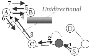
Figure 7: Routing failure caused by unidirectional links.
