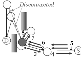
Figure 8: Routing failure caused by disconnected links.
