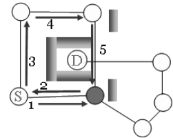
Figure 9: Routing failure caused by cross links.
