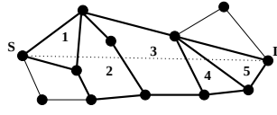
Figure 2: The faces progressively closer from S to D along line segment SD , numbered in the order visited. Faces cut by SD are bordered in bold.
