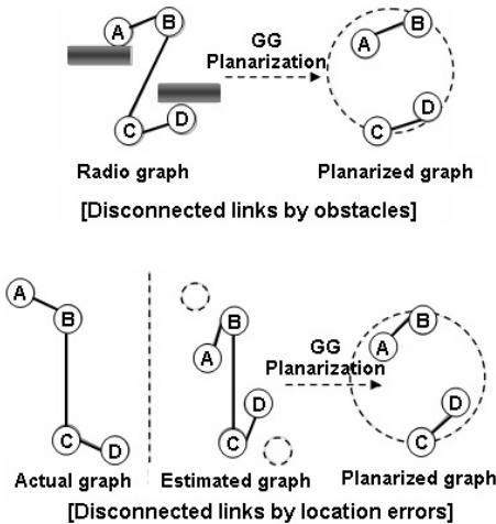
Figure 5: Disconnected links in subgraphs.
