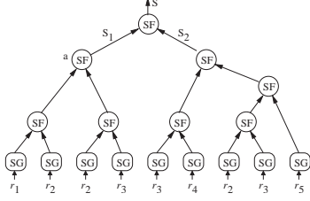
Figure 15: Graph used in the proof.
