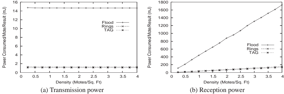
Figure 9: Impact of sensor density on power consumption.
