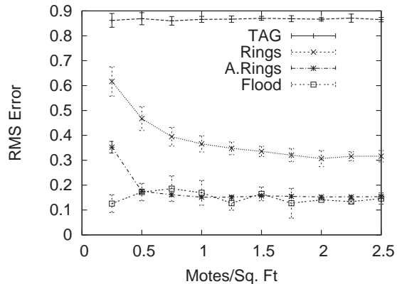
Figure 8: The impact of sensor density on accuracy.
