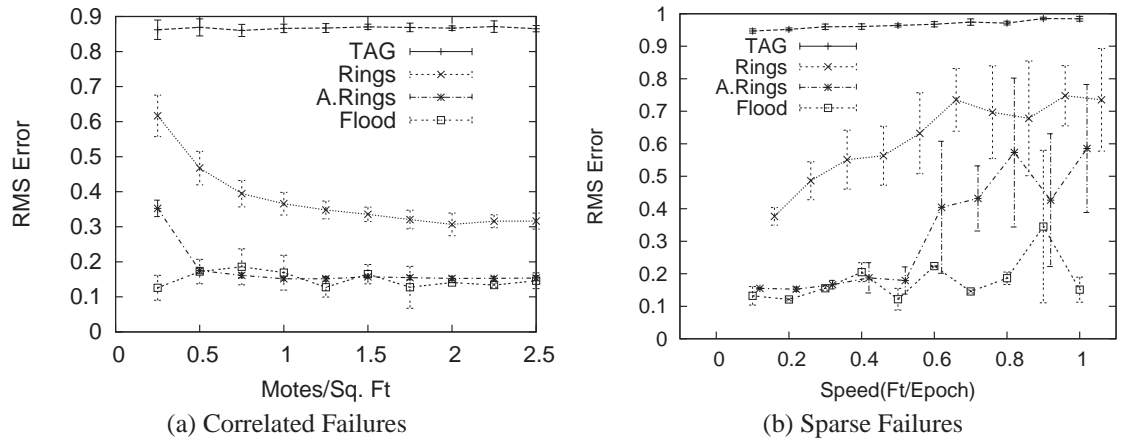
Figure 11: The effectiveness of the Adaptive Rings scheme to cope with node failures.
