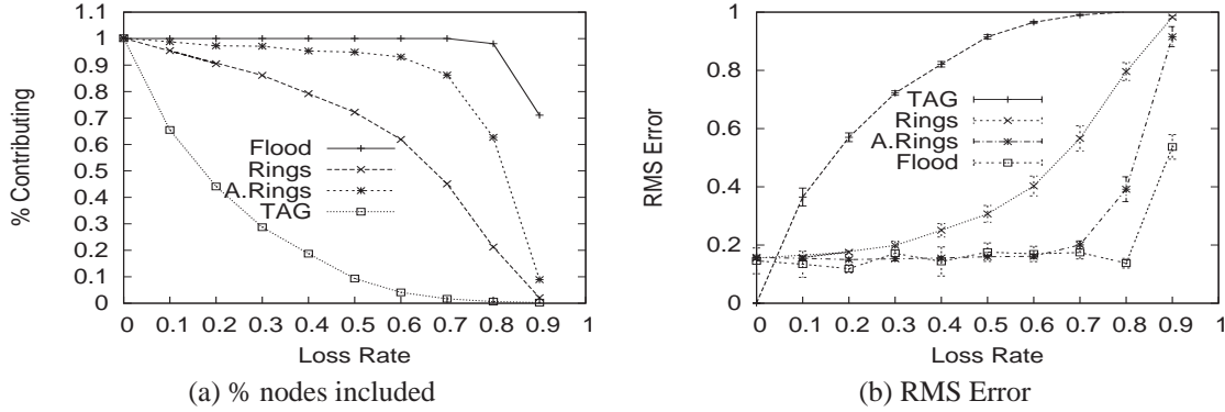
Figure 7: Impact of packet loss on aggregation schemes.
