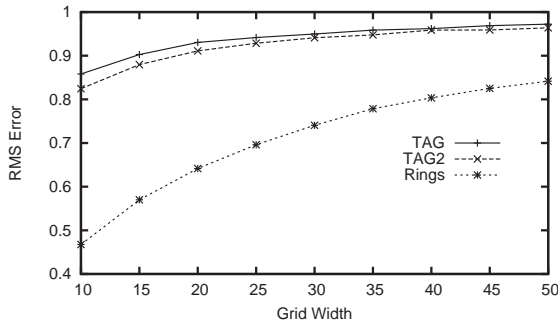
Figure 10: The impact of the shape of sensor deployment on accuracy.
