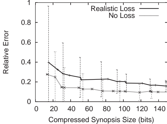
Figure 13: Effect of synopsis size in computing Sum
