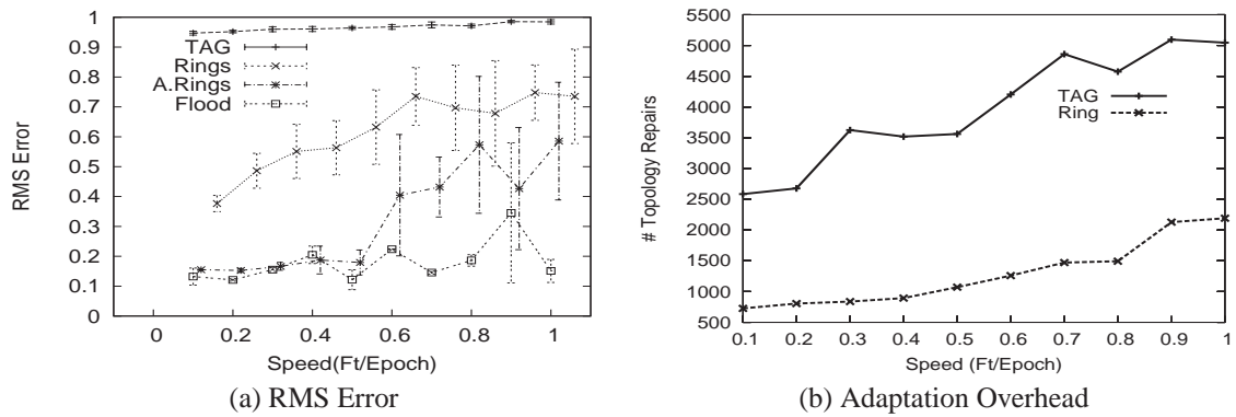
Figure 12: The impact of random motion on accuracy and topology adaptation overhead.
