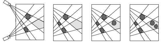
Figure 3: Different object arrangements can be consistent with a given visual hull. Polygons devoid of objects are called phantoms.
