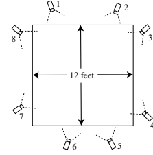
Figure 5: Top view of workspace with the cameras' FOV lines.
