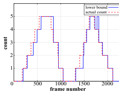
Figure 7: Count of 5 people walking into and out of the workspace.
