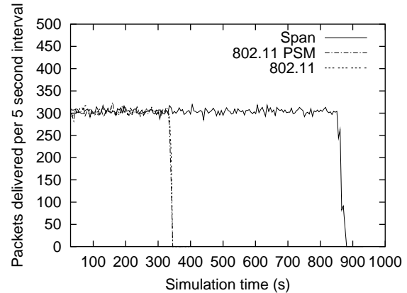
Figure 11: Packet delivery rate as a function of simulation time. This simulation ran on a 500\text{m} \times 500\text{m} area. With Span, the delivery rate does not drop below 90% until 851 seconds into the simulation, significantly longer than with 802.11 PSM and 802.11.
