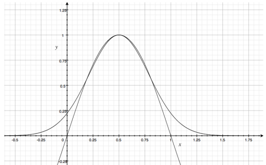
Figure 2: The half-sine pulse S ( \tau = 1 ) compared to a Gaussian approximation.
