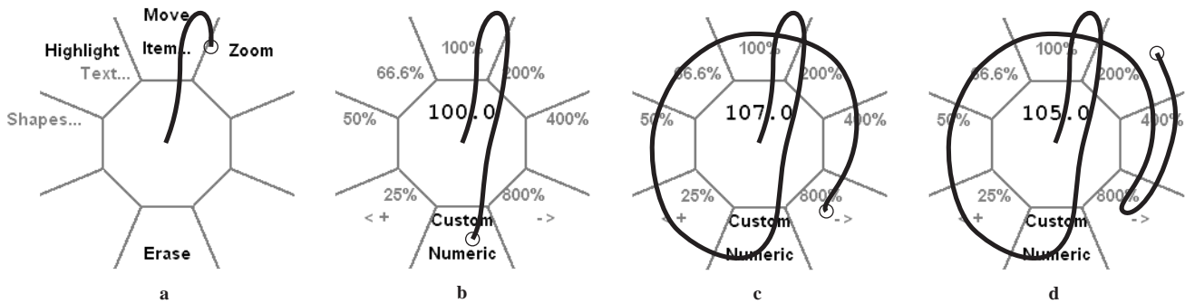
Figure 4: In this example, the knob interaction is used to adjust the zoom level. After selecting Item... → Zoom → Numeric (a,b), the user circles the pen around the center area, using the menu as a knob for fine adjustment. Each time an octant line is crossed, the value is incremented by a small amount (c) (decremented if counter-clockwise (d)). The zooming is done real-time, with the object visible (omitted in this figure for clarity) so visual feedback is provided at all times.
