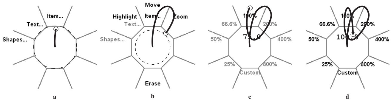
Figure 1: To zoom, the user moves the pen from the rest area into the Items... octant (a). Submenus ( Highlight , Move , Zoom ) appear and the first level menu items not selected are grayed out (b). Entering the Zoom octant submenu, then moving back to the rest area dismisses the root level menu and brings up the zoom menu with the current zoom value (75%) displayed in the center (c). A new zoom value of 100% is selected by moving into the octant for the desired value and back to the center at which point the zoom is applied (d). Several zoom values can be tried out during the same interaction since the zoom menu stays in place until the pen is lifted. The dashed circles added to the illustration (a) and (b) show the transition boundaries for leaving and entering the rest area (see text). For explanatory purposes, the figures in this paper explicitly show the pen track and the underlying selected object is shown only in Figure 3. In normal use, the pen track is not displayed and the selected object is visible behind the transparent menu.
