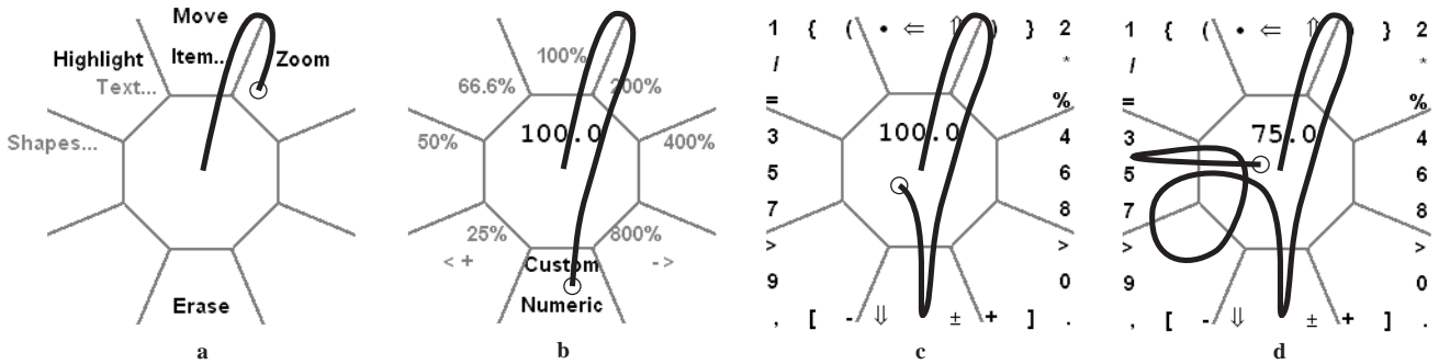
Figure 2: After selecting Item... → Zoom from the root menu (a), the user selects Numeric to enter the new zoom value as a sequence of digits (b). The zoom menu is dismissed and the Quikwriting system is brought up (c) so that she can enter the zoom value (d).
