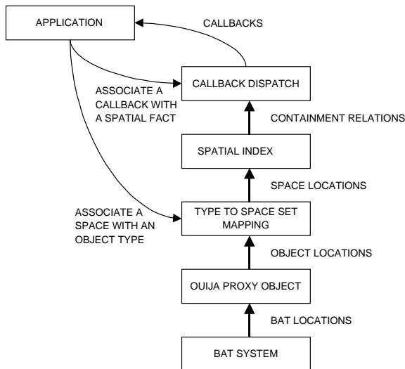
Figure 8: Transformation of absolute location events to application-centric callbacks
