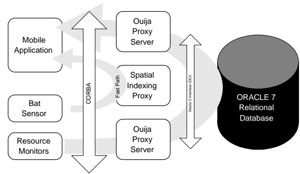
Figure 5: Three-tier architecture
