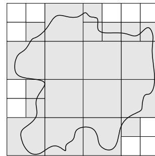
Figure 9: Maximal cover of a space
