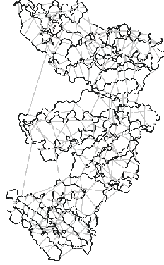
Figure 1. A spanner of a protein backbone. The spanner consists of the backbone edges (black) and a number of additional edges, the shortcuts (light gray). There is a path between any two backbone atoms with length at most 3 times their Euclidean distance.
