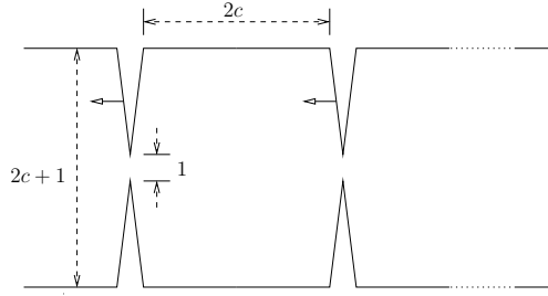
Figure 7. Lower bound \Omega(n^2/c^2) for the changes of any linear-size spanner.
