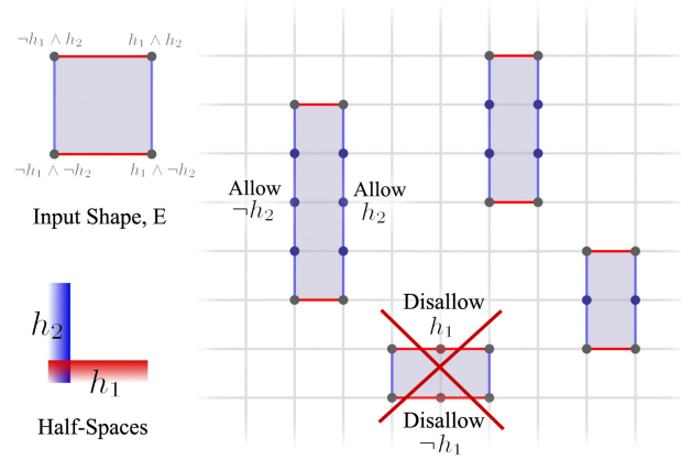
Fig. 6. Dimensional Constraint. To create objects that are only one plane space wide horizontally, we disallow any states which pass through the vertical h_2 planes such as h_1 or \sim h_1 .
