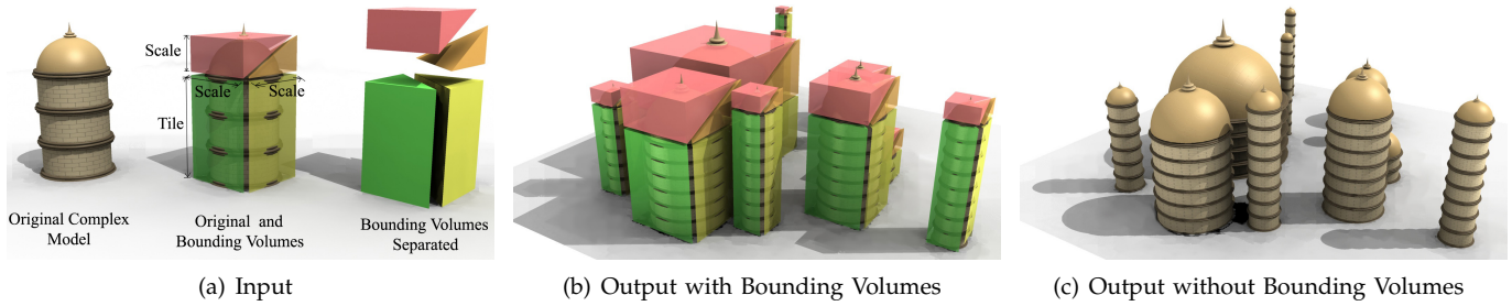
Fig. 7. Because model synthesis is inefficient on curved models bounding volumes are used to simplify the geometry (a). The bounding boxes are cut into two objects, so the dome will scale uniformly and the cylinder will scale uniformly in x and y . The output is generated and the complex original shapes are substituted back in (b,c).
