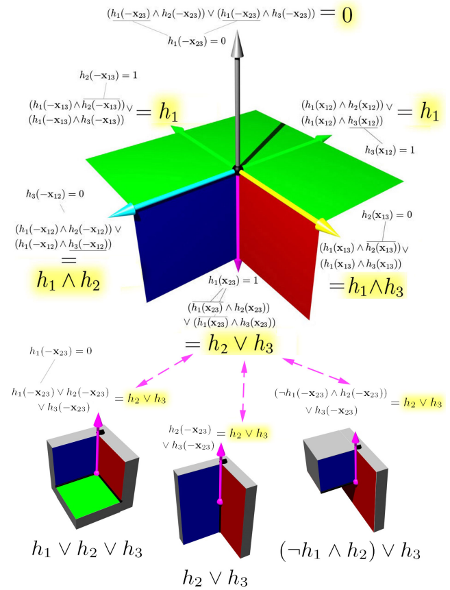
Fig. 4. We can evaluate the states to figure out which states can be adjacent to them in various directions. This shows the state (h_1 \wedge h_2) \vee (h_1 \wedge h_3) evaluated in six directions. We assume that \mathbf{x}_{23} points down and is inside the h_1 half-space so that h_1(\mathbf{x}_{23}) = 1 and h_1(-\mathbf{x}_{23}) = 0 . In the \mathbf{x}_{23} direction, the state (h_1 \wedge h_2) \vee (h_1 \wedge h_3) evaluates to h_2 \vee h_3 which is shown as the magenta edge. A state can only be underneath the state (h_1 \wedge h_2) \vee (h_1 \wedge h_3) if it shares the same h_2 \vee h_3 edge. We test every state to see which ones evaluate to h_2 \vee h_3 in the -\mathbf{x}_{23} direction. Three acceptable states are shown: h_1 \vee h_2 \vee h_3 , h_2 \vee h_3 , and (\neg h_1 \wedge h_2) \vee h_3 .
