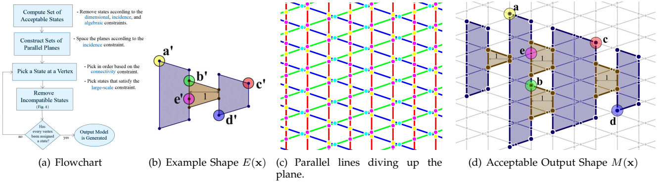
Fig. 2. (a) Overview flowchart showing how the constraints affect the algorithm. (b) From the input shape E , (c) sets of lines parallel to E intersect to form edges and vertices. (d) The output shape is formed within the parallel lines. For each selected point a , b , c , d , and e in M , there are points a' , b' , c' , d' , and e' in the example model E which have the same neighborhood. The models E and M contain two different kinds of object interiors shown in blue and brown. The brown object's width is constrained to be one line spacing width. The width of the blue object is not constrained. The objects are also constrained to be fully connected.
