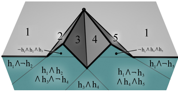
Fig. 5. Even complex vertices can be described using a Boolean expression of half-spaces. We can take all the faces that intersect the vertex and use all of the planes the faces are on to divide up the space into regions that are the intersection of several half-spaces. The regions labeled in the figure are inside the polyhedron. The vertex state is described as the union of all these interior regions. This vertex is simplified to (h_3 \wedge (h_1 \vee h_2)) \vee (h_4 \wedge (h_1 \vee h_5)) .
