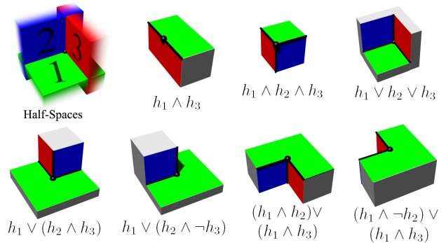
Fig. 3. One edge and six vertex states are described using Boolean expressions of three half-spaces. In our algorithm, every neighborhood is represented by a Boolean expression.
