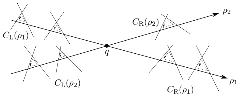
Figure 7: The structure of the double wedge W(\rho_1, \rho_2) and the cycles along it
