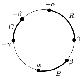
Figure 6: Illustration of condition (C2); B, R, G are used to label the intervals containing the directions of the corresponding projected lines
