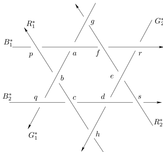
Figure 3: The Magen-David weaving
