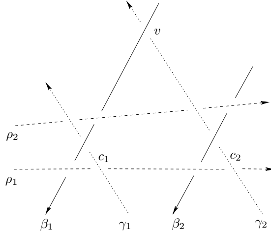
Figure 8: The blue-green vertex v must lie in W(\rho_1, \rho_2)
