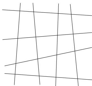
Figure 2: A collection of line segments that forms a grid
