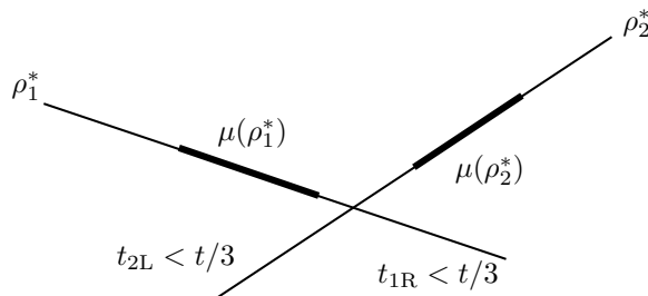
Figure 9: \mu(\rho_1^*) and \mu(\rho_2^*) lie on the upper envelope of \rho_1^*, \rho_2^*
