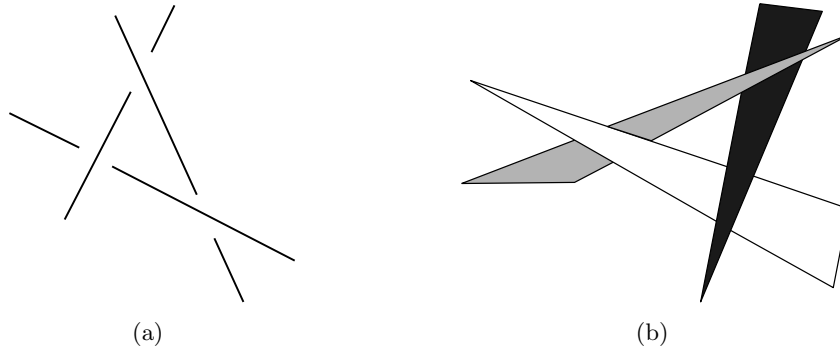
Figure 1: Depth cycles formed (a) by three lines and (b) by three triangles
