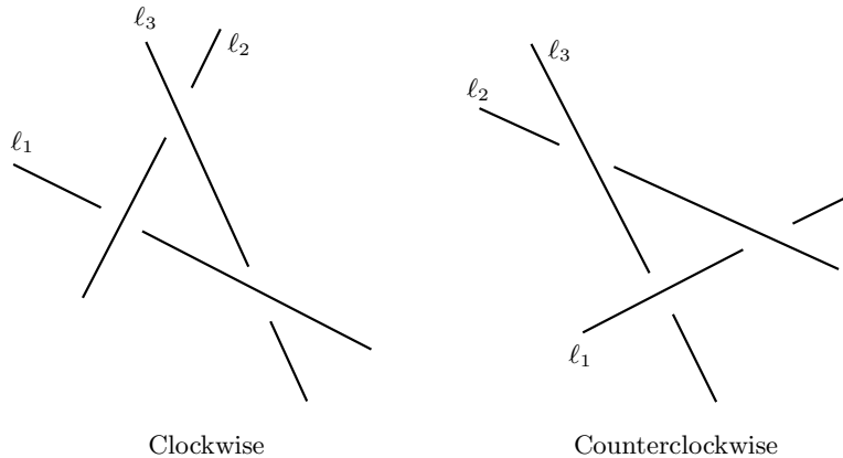
Figure 5: The two types of triangular cycles
