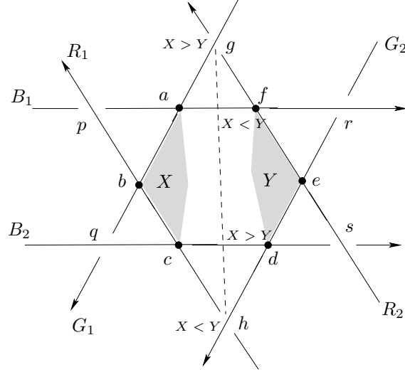
Figure 4: An (impossible) realization of the Magen-David weaving, after six contacts were enforced
