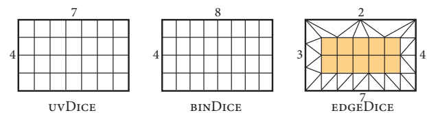
Figure 3: Comparison of dicing methods: The Reyes dicer (UV DICE) accepts tessellation factors for the patch’s u and v parametric directions. It produces a uniform mesh tessellation according to these factors. Binary UV dice only tessellates each edge using a power-of-two number of segments. The D3D11 tessellator (EDGEDICE) can accommodate per edge factors. Each edge of the patch is tessellated uniformly with a number of segments equal to the provided factor. The EDGEDICE scheme “stitches” a uniformly tessellated interior mesh to segments along the edges.
