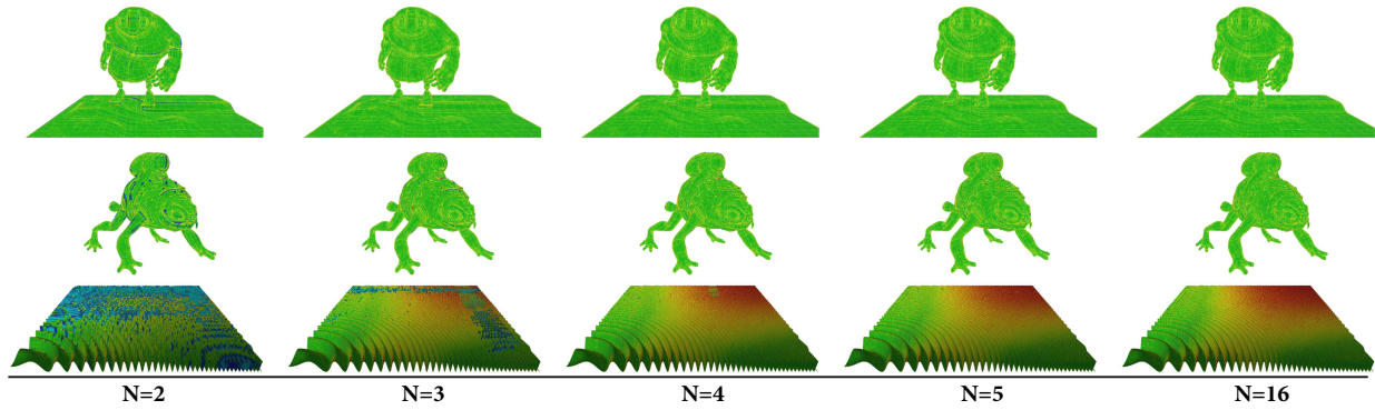
Figure 11: DIAGSPLIT tessellation quality improves as the number of surface samples used by \mathcal{T} increases. Errors due to sparse edge sampling are particularly apparent in ZONEPLATE, which contains a surface with high frequency detail. Our implementation of DIAGSPLIT uses four samples to determine the tessellation factor for an edge ( N=4 ).
