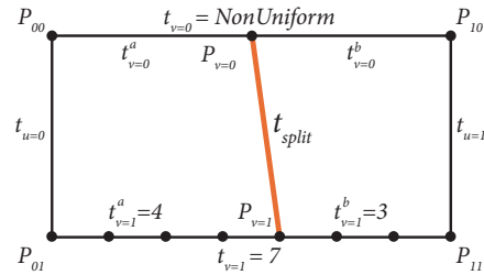
Figure 7: DIAGSPLIT's splitting algorithm: The function DiagSplit takes four parametric coordinates that define an input patch and emits subpatches that, when diced, contain micropolygons with near-uniform area.
