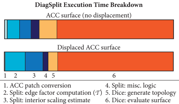
Figure 12: Relative cost of major DIAGSPLIT operations when tessellating MONSTERFROG with and without displacement. Dicing dominates execution time of computing a DIAGSPLIT tessellation.
