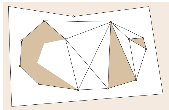
Fig. 5.6 The shortest-path roadmap includes edges between consecutive reflex vertices on \mathcal{C}_{\text{obs}} and also bitangent edges
