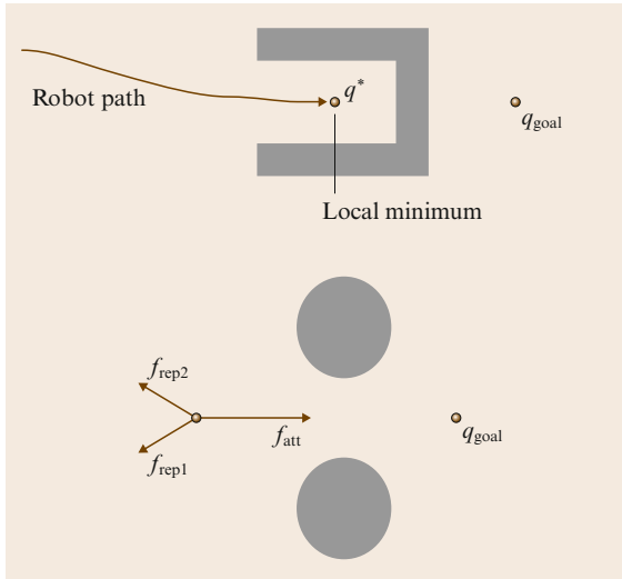
Fig. 5.9 Two examples of the local minimum problem with potential functions
