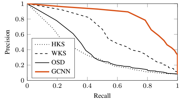
Figure 8: Performance (in terms of Precision-Recall) of shape retrieval on the FAUST dataset using different descriptors. Higher curve corresponds to better performance.
