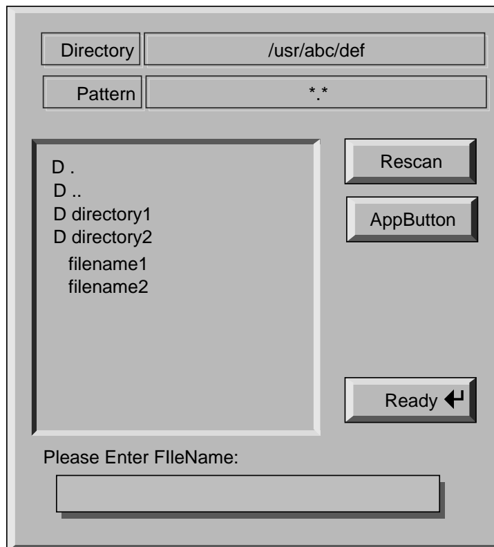
Figure 6.1: File selector
