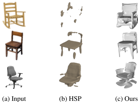
Figure 6. Single-view reconstruction comparison on natural images. From a 2D RGB image taken from internet (a), HSP [13] reconstructs a octree-based 3D model (b), and our AtlasNet a triangular mesh (c).
