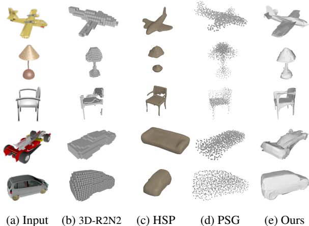
Figure 5. Single-view reconstruction comparison. From a 2D RGB image (a), 3D-R2N2 [7] reconstructs a voxel-based 3D model (b), HSP [13] reconstructs a octree-based 3D model (c), PointSetGen [9] a point cloud based 3D model (d), and our AtlasNet a triangular mesh (e).
