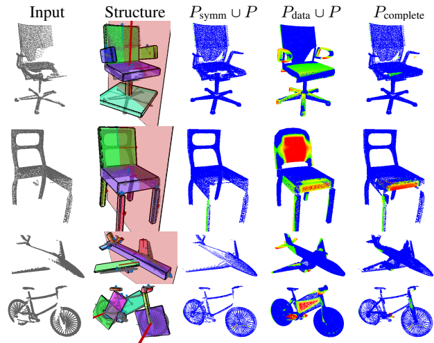
Figure 7: This figure demonstrates our shape completion results: input point cloud, estimated structure, symmetry-only completion accuracy, data-base only completion accuracy, and the final combined result. Note how symmetry-only completion consistently leaves large blank regions, and database-driven approach hallucinates pieces of geometry that should not be there (see red regions). In contrast, our method effectively combines both priors to produce accurate and complete shapes.
