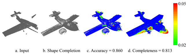
Figure 5: This figure demonstrates our evaluation technique. Given the input point cloud (a), we run our algorithm to complete the shape (b), and then evaluate accuracy and completeness. The accuracy image (c) colors the points of the completed shape based on the distance to the nearest point on the true shape (see error bar on the right). The completeness image (d) colors the points of the true shape based on the distance to the nearest point on the completed shape. See supplemental material for the results on the entire benchmark.
