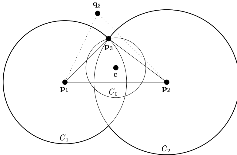
Figure 2: Illustration of Lemma 1.
