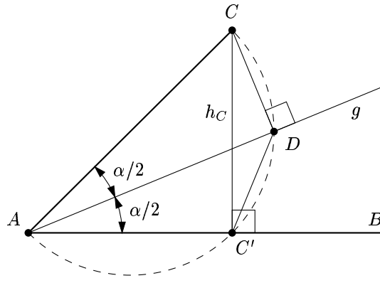
Figure 14: Proof of Lemma 22
