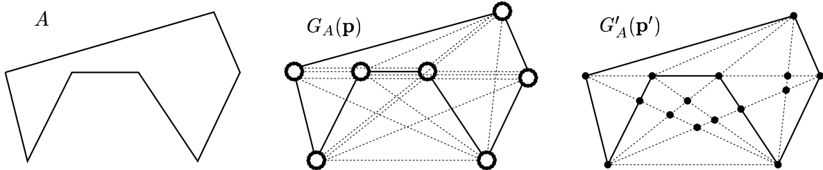
Figure 4: Construction of the frameworks G_A(\mathbf{p}) and G'_A(\mathbf{p}') . Solid lines denote bars, and dashed lines denote struts.
