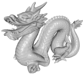
(a) The Stanford dragon, a surface represented by 3.2 million triangles. It has no holes, but 60 tunnels.
